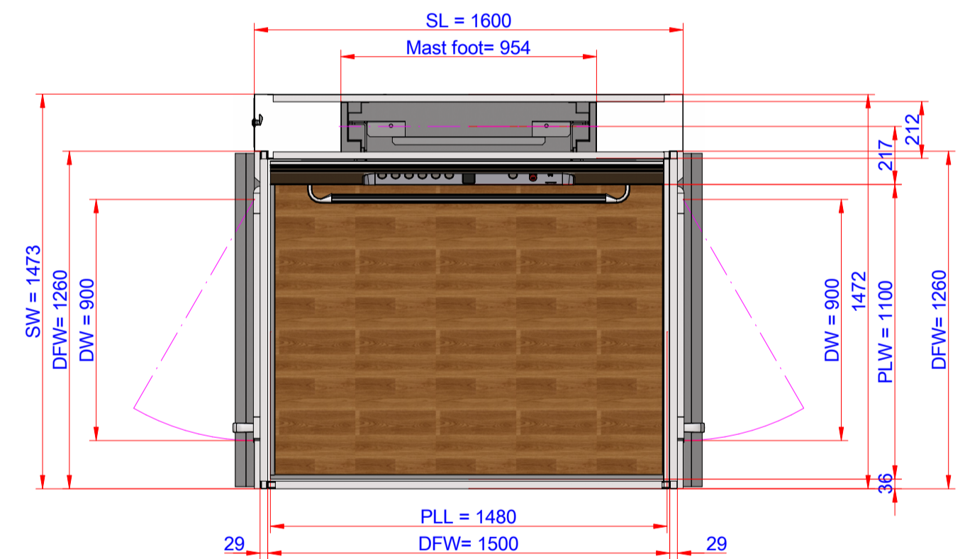
PLAN VIEW Scale: 1:20
